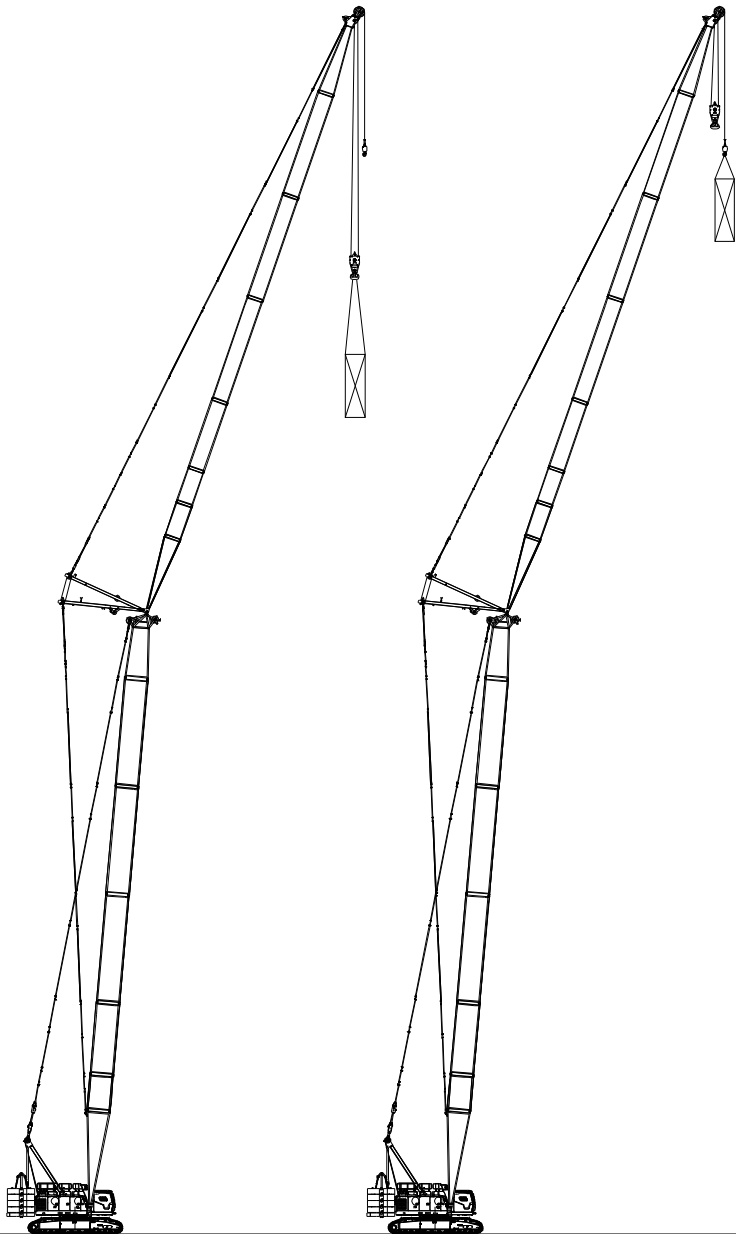
LJ Configuration (double hooks, load on luffing jib hook) LJa Configuration (double hooks, load on extension jib hook)
